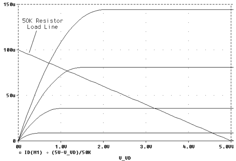
Figure 65 Operating Point Determination for Each Member of the Curve Family
