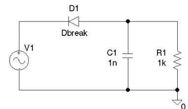
Figure 31 Schematic for a Half-Wave Rectifier
