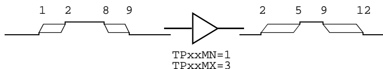
Figure 110 Cumulative Ambiguity Hazard Example 1
