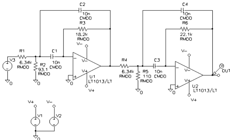
Figure 87 Chebyshev Filter
