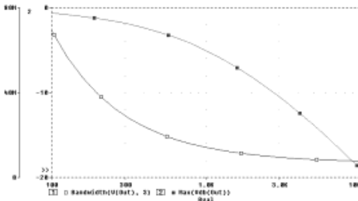
Figure 27 Performance Analysis Plots of Bandwidth and Gain vs. Rval
