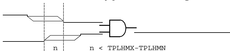
Figure 116 Glitch Suppression Example 2
