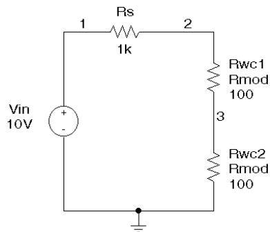
Figure 96 Schematic Demonstrating Use of VARY BOTH
