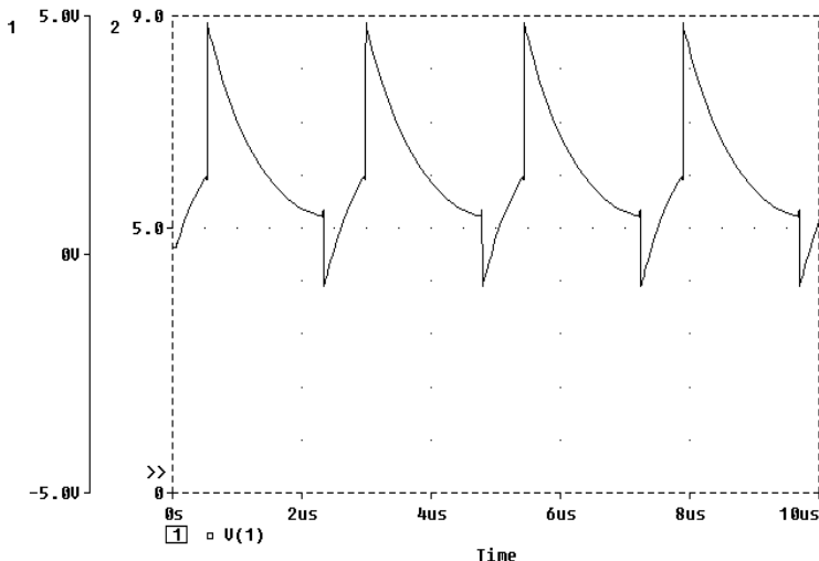
Figure 126 Voltage at net 1 with y-axis added.
