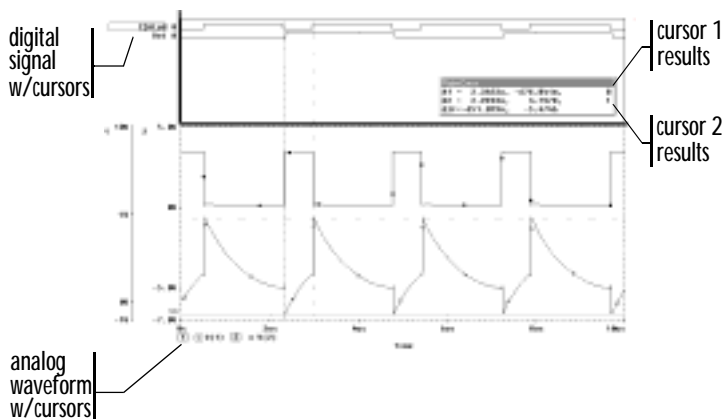
Figure 128 Cursors positioned on a trough and peak of V(1)
