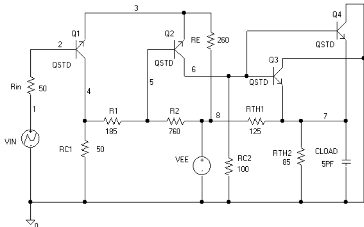
Figure 70 ECL Compatible Schmitt Trigger
