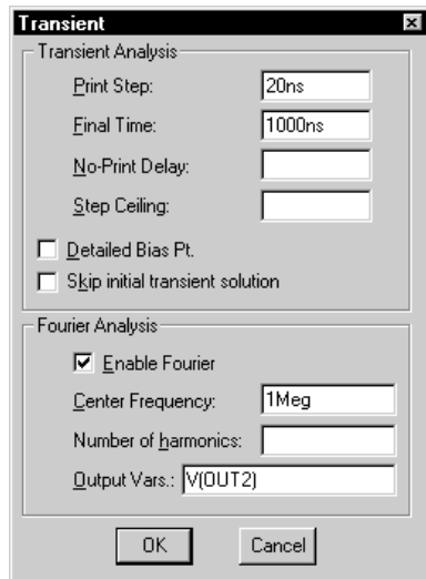
Figure 68 Transient Analysis Setup for example.sch
