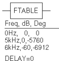
Figure 42 FTABLE Part Example
