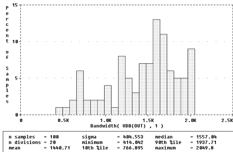
Figure 89 1 dB Bandwidth Histogram
