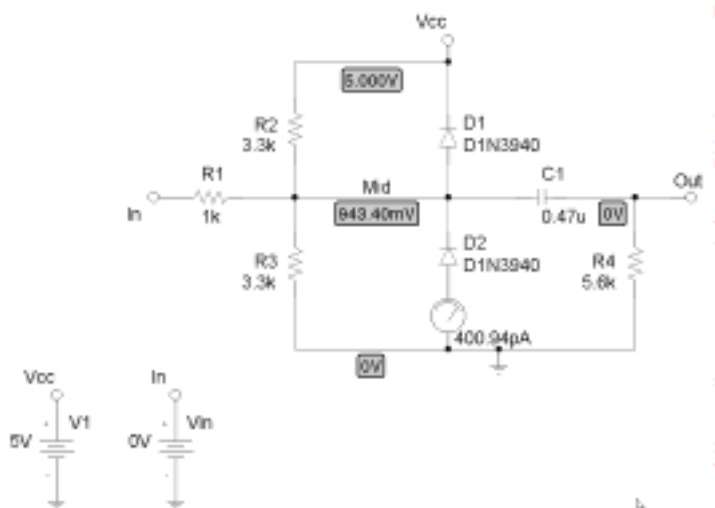
Figure 5 Clipper Circuit with Bias Point Voltages Displayed
