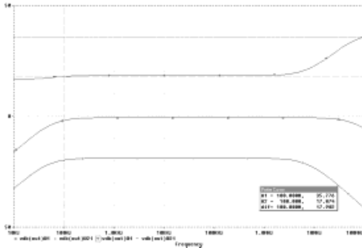
Figure 26 Comparison of Small Signal Frequency Response at 100 and 10 k \Omega Input Resistance
